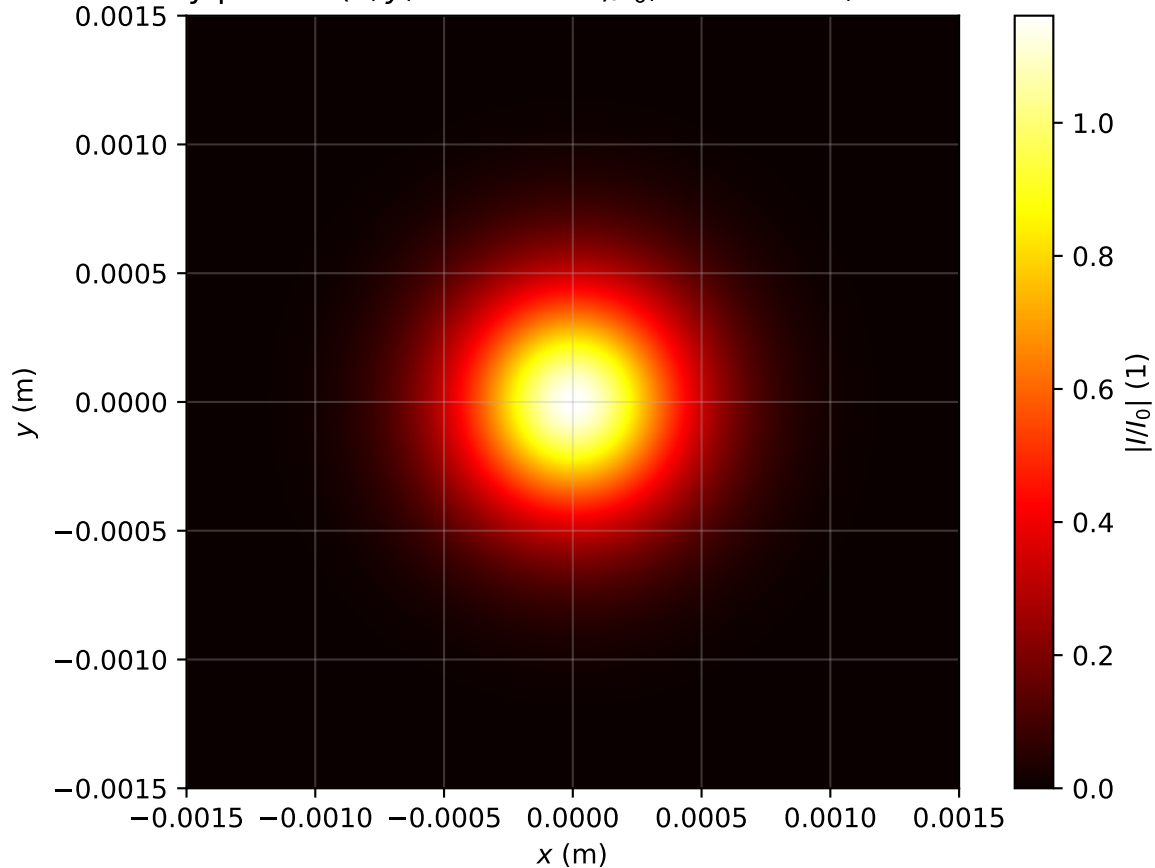
Intensity profile I(x, y, z = 0.478m)/I_0 , P_{in}=1.0P_{cr} , artificial time
